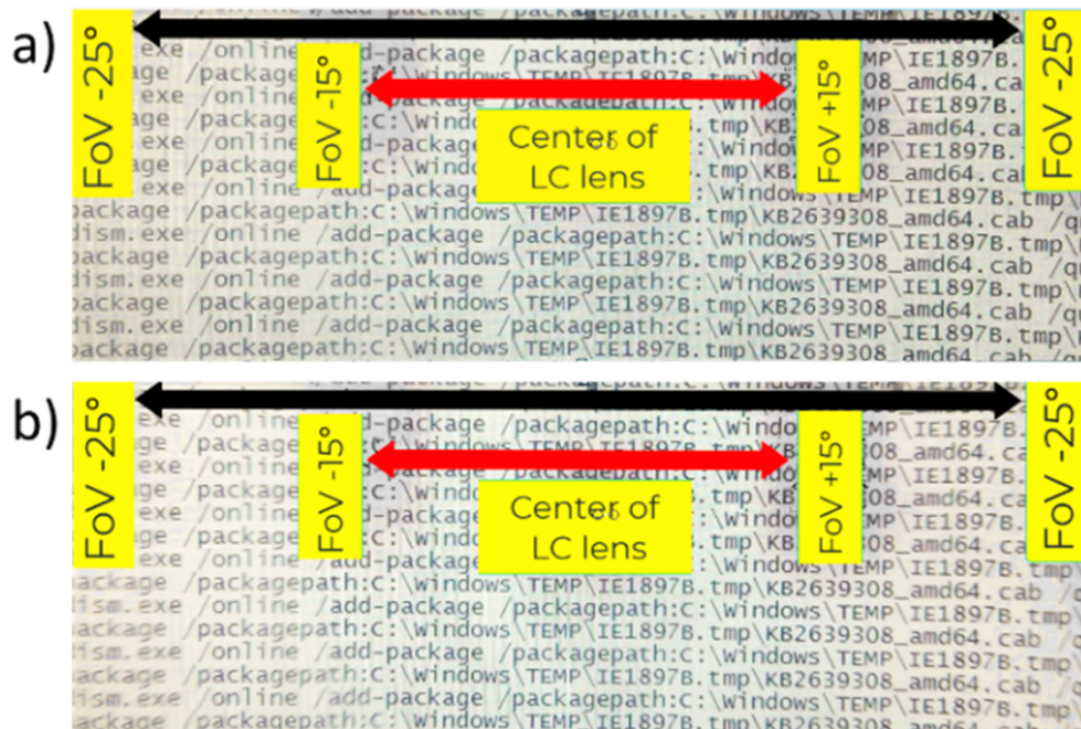
Fig. 9: Optical quality evaluation images on a lab-based VR system, a) LC lens is off for case-1, b) LC lens at +0.80 D for on axis view with +/- 25 degrees gaze angle. (note: the camera is refocused as the lens power changes)
