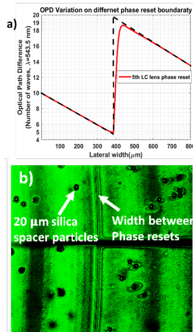
Fig. 3 a) Simulated phase resets of the LC lens (red) compared to ideal Fresnel reset (black dashed line), b) closer look at the phase profile to show width of phase distortion correlates with cell spacer thickness.
