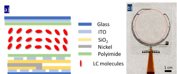
Fig.1: a) Side view of inner layer structure of the device, b) fabricated single 5 cm aperture LC lens, red dashed border on the image representing the lens area.
