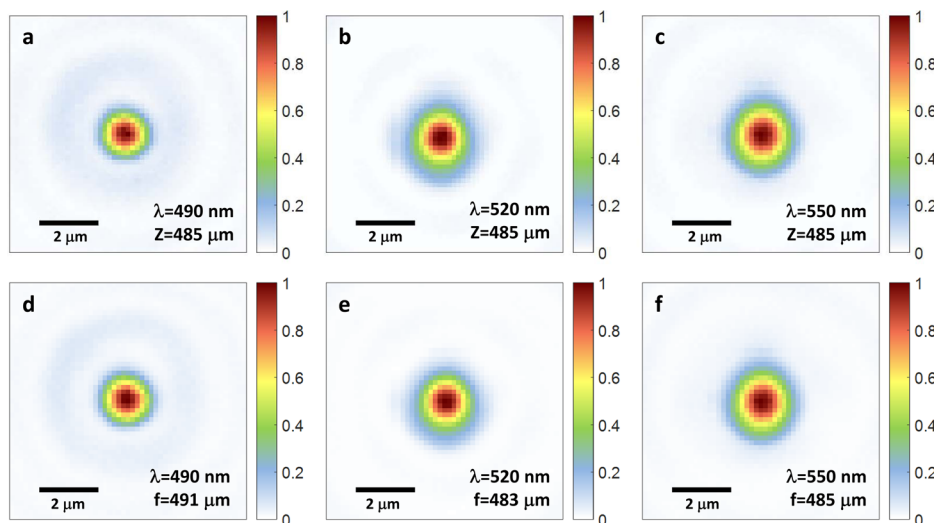
Figure 5. Top row: measured intensity profiles of the AML at a fixed position of z = 485 \mu\text{m} at three wavelengths of (a) 490, (b) 520, and (c) 550 nm. Bottom row: measured focal spots of the AML at three wavelengths of (d) 490, (e) 520, and (f) 550 nm. The vertical (horizontal) cuts of focal spots have a full width at half-maximum (fwhm) of 1.27 \mu\text{m} ( 1.29 \mu\text{m} ), 1.52 \mu\text{m} ( 1.45 \mu\text{m} ), and 1.68 \mu\text{m} ( 1.59 \mu\text{m} ) at wavelength of 490, 520, and 550 nm, respectively. Values of fwhms from vertical and horizontal cuts are very close revealing the symmetry of the focal spots.
