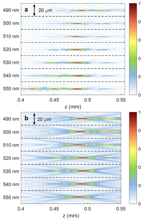
Figure 4. (a) Measured intensity profiles of the reflected beam by the AML in the xz -plane at different wavelengths. Wavelength of the incident light is noted in the left side of the plot. Focal spots of the AML at the different wavelengths appear at the same z distance from the AML. The variation of focal length across the wavelength range of 490–550 nm is negligible with a standard deviation of 2.7 \mu\text{m} . (b) Simulated intensity profiles of the reflected beam by the AML in the xz -plane at different wavelengths.
