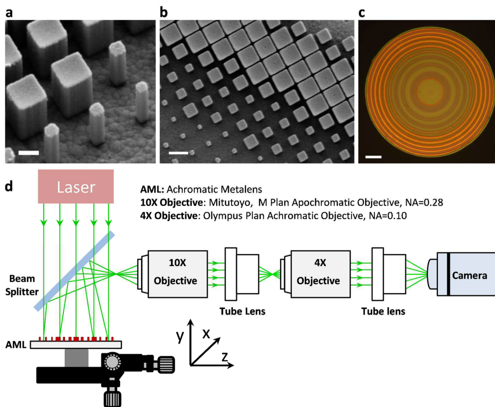
Figure 3. (a) Side-view scanning electron microscope (SEM) image of the fabricated AML. Scale bar: 200 nm. (b) Top-view SEM image of the AML. Scale bar: 500 nm. (c) Optical image of the AML. Scale bar: 25 μm. (d) Schematic of custom-built setup used to characterize the AML. The AML reflects and focuses the collimated incident light. We cascaded two objectives to increase the imaging magnification to 40.
