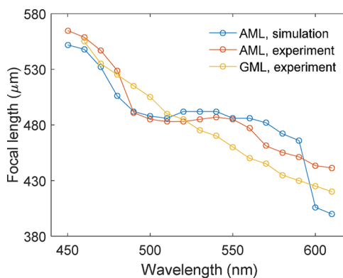
Figure 2. AML, simulation: calculated focal length of the AML as a function of wavelength. AML, experiment: measured focal length of the fabricated AML versus wavelength. The measured fractional change of focal length across the bandwidth (490–550 nm) is 1.5% very close to that of predicted by simulation (1.2%). The AML has a diameter of 200 \mu\text{m} and focal length of 485 \mu\text{m} at \lambda = 530 nm. Geometric-phase-based metalens (GML), experiment: measured focal length of a fabricated GML. The required phase is imparted via the rotation of titanium dioxide nanofins. The use of geometric phase has a high tolerance to fabrication errors thus GML can serve as a robust reference.
